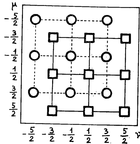
FIG. 1. The density matrix \rho^{(F)} for spin \frac{5}{2} . The elements indicated by circles form the matrix \rho' , those indicated by squares form the matrix \rho'' .
